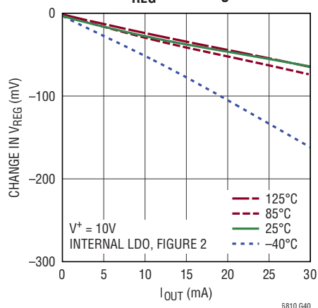
Internal V REG Load Regulation
