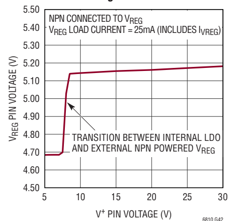
V REG Pin Voltage vs V + Pin Voltage
