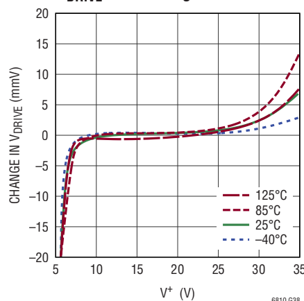
V DRIVE V + Line Regulation
