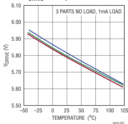
V DRIVE vs Temperature
