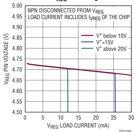
Internal V REG Load Regulation
