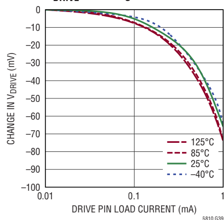
V DRIVE Load Regulation
