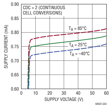
Supply Current vs Supply Voltage in CDC = 2
