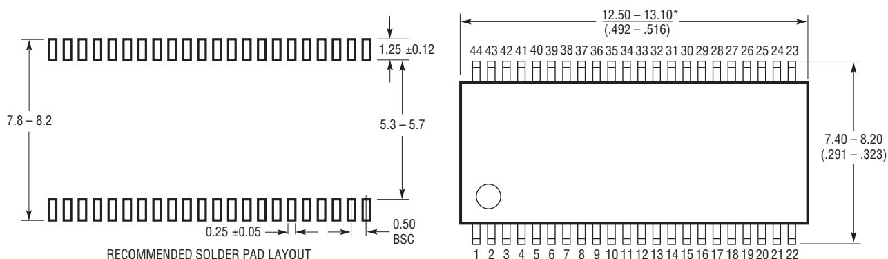
G Package 44-Lead Plastic SSOP (5.3mm) (Reference LTC DWG # 05-08-1754 Rev A)
