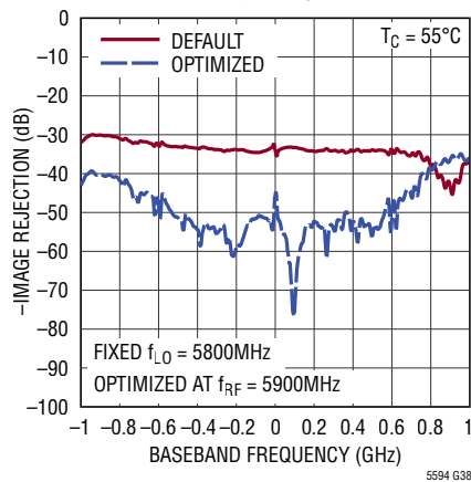
Optimized Image Rejection vs Baseband Frequency
