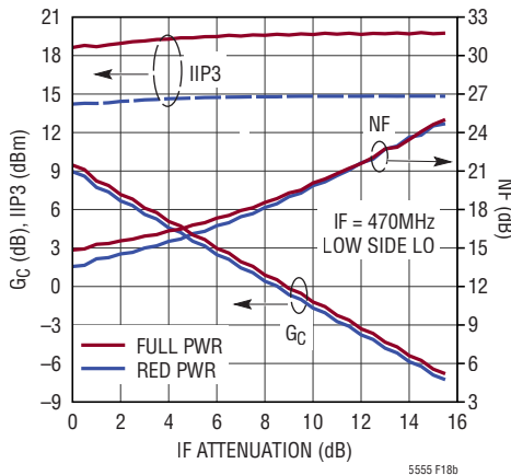
6.5GHz Conv Gain, IIP3, and SSB NF vs IF Attenuation (0.5dB Steps)
