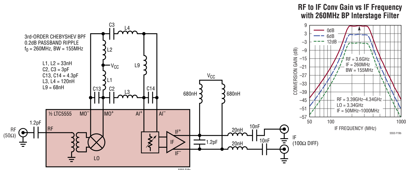
Figure 20. Test Circuit and Measured Conversion Gain with 3rd-Order Bandpass Interstage Filter
