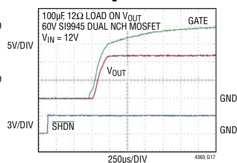
Turn-On Timing
