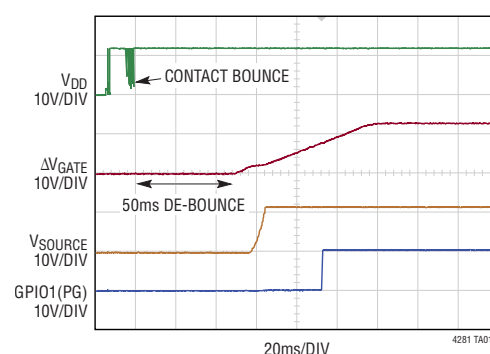
Start-Up Waveforms
