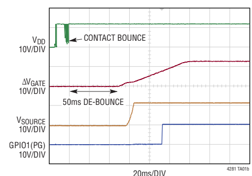
Start-Up Waveforms
