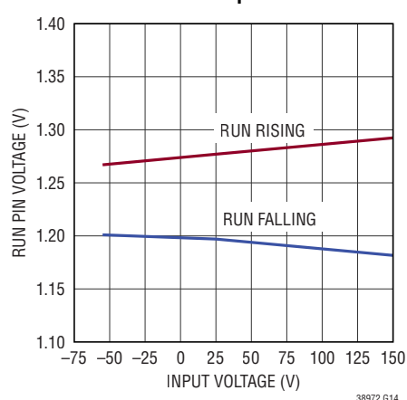
BOOST Shutdown (RUN) Threshold vs Temperature
