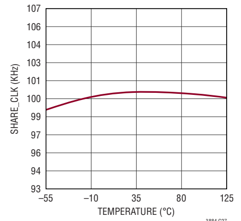
SHARE_CLK vs Temperature
