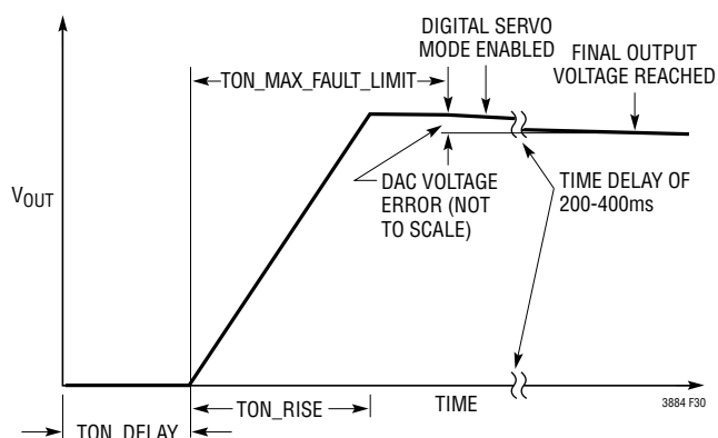
Figure 30. Timing Controlled V_{\text{OUT}} Rise
