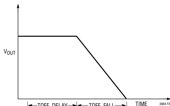
Figure 31. \text{TOFF\_DELAY} and \text{TOFF\_FALL}
