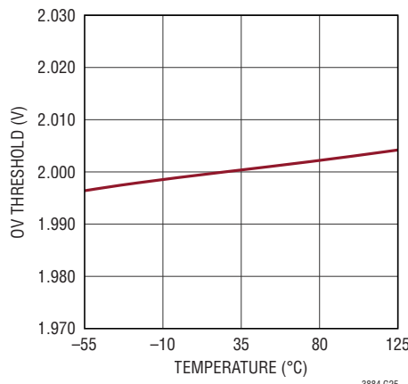
V OUT Overvoltage Threshold vs Temperature (Target 2V)
