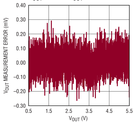
V_{OUT} Error vs V_{OUT}
