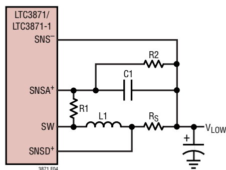
Figure 4. R SENSE Resistor Sensing
