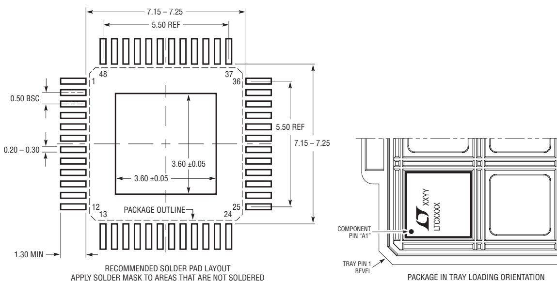
PACKAGE IN TRAY LOADING ORIENTATION
