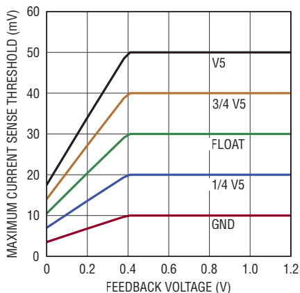
Maximum Current Sense Threshold vs Feedback Voltage (DCR) (LTC3871-1)
