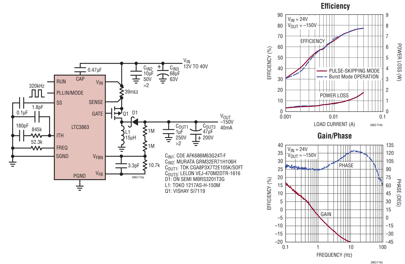
Figure 16. 12V to 40V Input, -150V/40mA Output, 320kHz Inverting Converter
