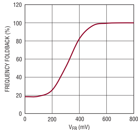
Frequency Foldback % Over Feedback Voltage
