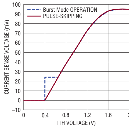
Current Sense Voltage Over ITH Voltage
