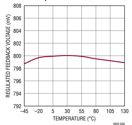
Buck Regulated Feedback Voltage vs Temperature
