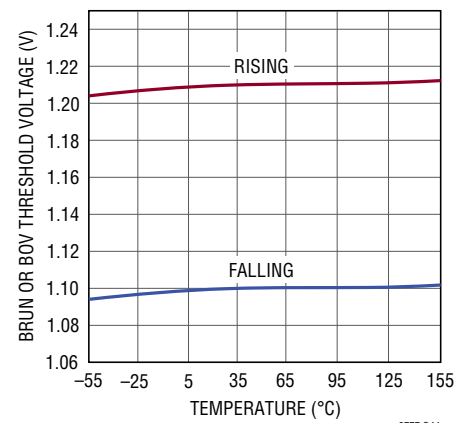
BRUN and BOV Comparator Threshold vs Temperature
