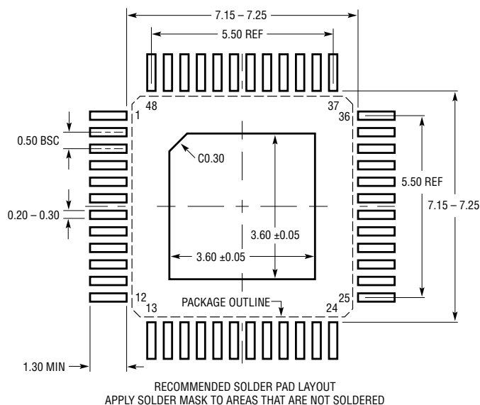
LXE Package 48-Lead Plastic Exposed Pad LQFP (7mm × 7mm) (Reference LTC DWG #05-08-1832 Rev D)
