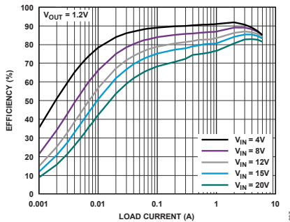
Figure 5. Efficiency vs Load Current Burst Mode Operation
