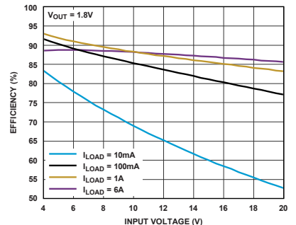
Figure 6. Efficiency vs Input Voltage Burst Mode Operation
