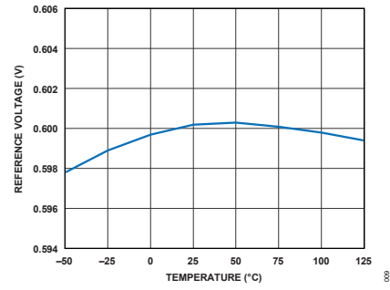
Figure 7. Reference Voltage vs Temperature
