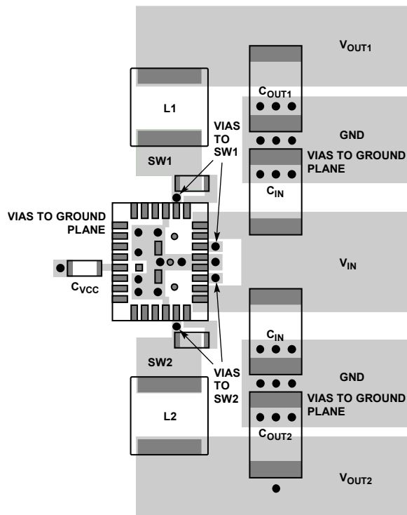
Figure 36. Recommended PCB Layouts - Alternative Layout with GNDT Pins Connected to GND
