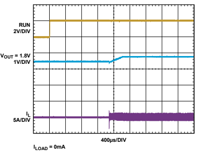
Figure 21. Start-Up (Burst Mode Operation)
