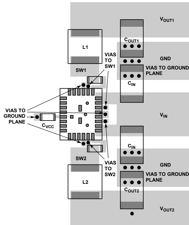
Figure 37. Recommended PCB Layouts - Alternative Layout with Pins 29 to 34 Unconnected
