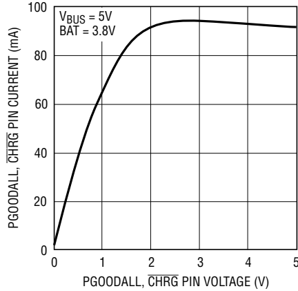
PGOODALL, \overline{\text{CHRG}} Pin Current vs Voltage (Pull-Down State)
