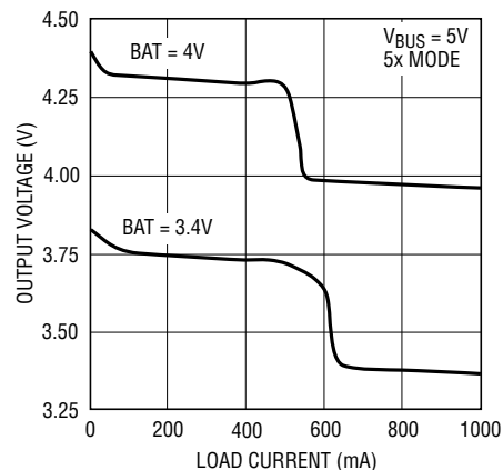
Output Voltage vs Load Current (Battery Charger Disabled)
