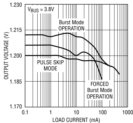
Switching Regulators 1, 2 Load Regulation at V_{\text{OUT1,2}} = 1.2\text{V}
