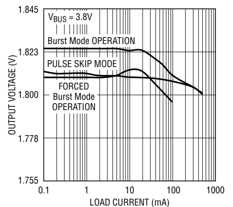
Switching Regulators 1, 2 Load Regulation at V_{\text{OUT1,2}} = 1.8\text{V}
