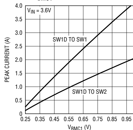
OUT1 Minimum Peak Current vs V_{BMC1}
