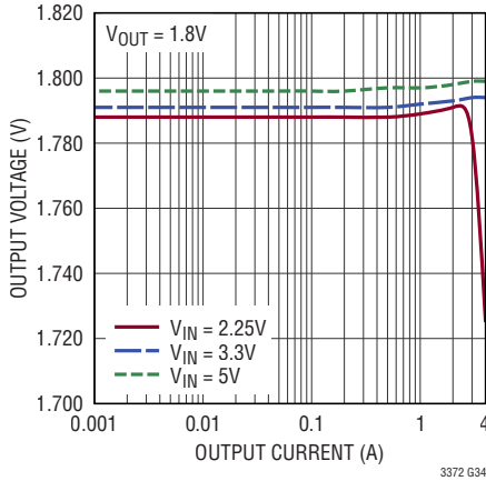
4A Buck Output Voltage vs Output Current
