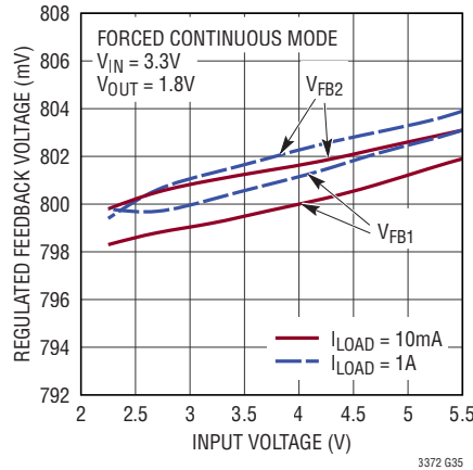
2A Buck Regulated Feedback Voltage vs V_{INA-H}
