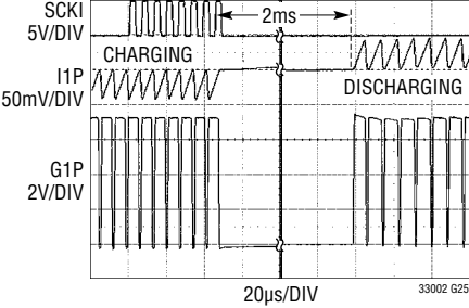
Changing Balancer Direction "On the Fly"
