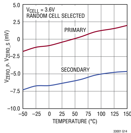
Zero Current Sense Threshold vs Temperature
