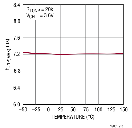
Primary Winding Switch Maximum On-Time vs Temperature
