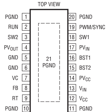
FE PACKAGE 20-LEAD PLASTIC TSSOP T_{JMAX} = 150^{\circ}\text{C} , \theta_{JA} = 38^{\circ}\text{C/W} , \theta_{JC} = 10^{\circ}\text{C/W} EXPOSED PAD (PIN 21) IS PGND, MUST BE SOLDERED TO PCB FOR RATED THERMAL PERFORMANCE
