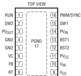
DHD PACKAGE 16-LEAD (5mm × 4mm) PLASTIC DFN T_{JMAX} = 125^{\circ}\text{C} , \theta_{JA} = 43^{\circ}\text{C/W} , \theta_{JC} = 4.3^{\circ}\text{C/W} EXPOSED PAD (PIN 17) IS PGND, MUST BE SOLDERED TO PCB
