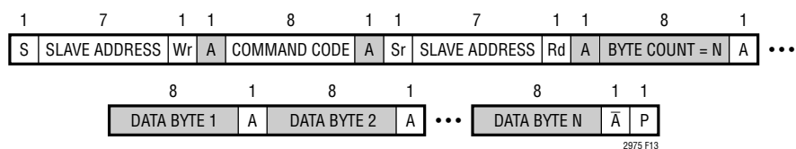
Figure 13. Block Read
