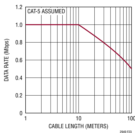
Figure 24. Data Rate vs Cable Length
