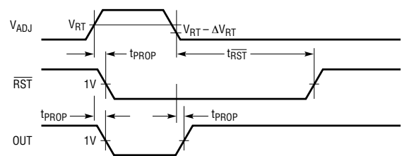
Negative Polarity Input Timing
