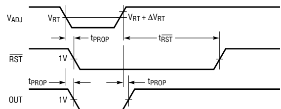
Positive Polarity Input Timing
