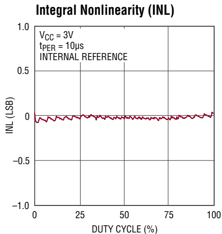
LTC2644-8 (Internal Reference, V_{FS} = 2.5\text{V} )
