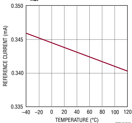
Reference Current vs Temperature, V_{\text{REF}} = 4.096\text{V}
