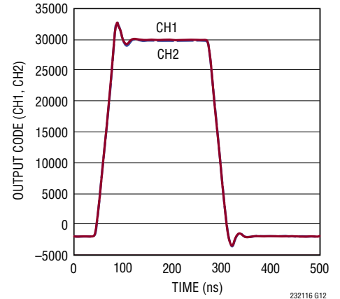
Output Match with Simultaneous Input Steps at CH1, CH2
