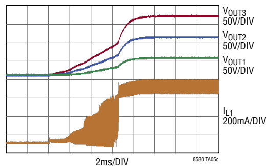
Start-Up Waveforms
