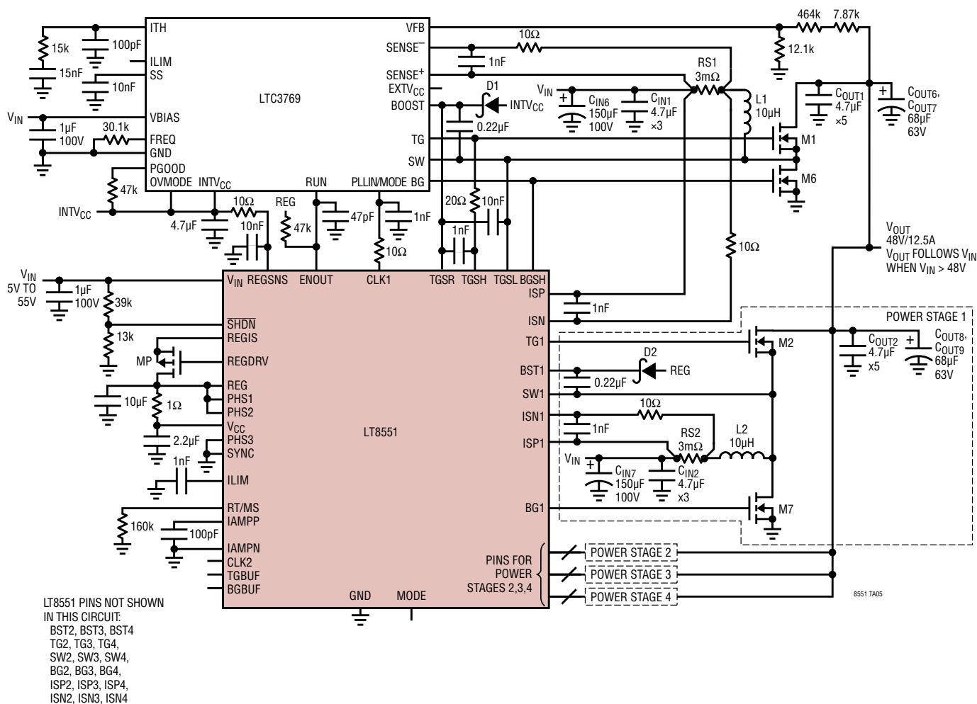
48V/12.5A Step-Up Expander System
