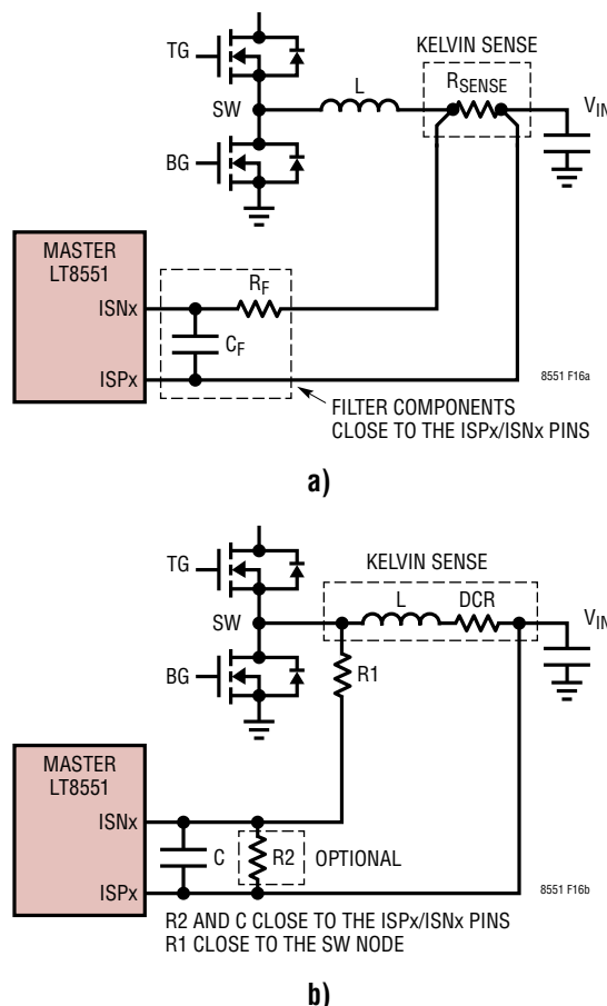
Figure 16. Inductor Current Sense Filter
