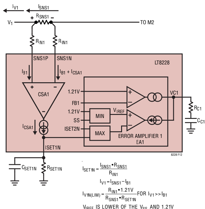
Figure 12. V_1 Output Current Limit Programming at ISET1N
