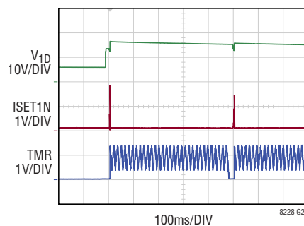
Output Short (Boost, Start-Up)
