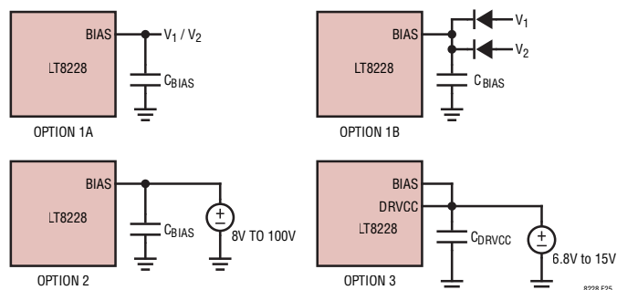
Figure 25. Possible Connections of BIAS Pin
