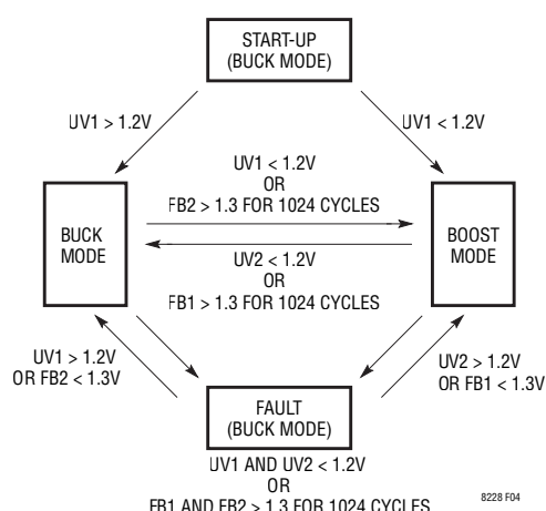
Figure 4. Automatic Mode of Operation
