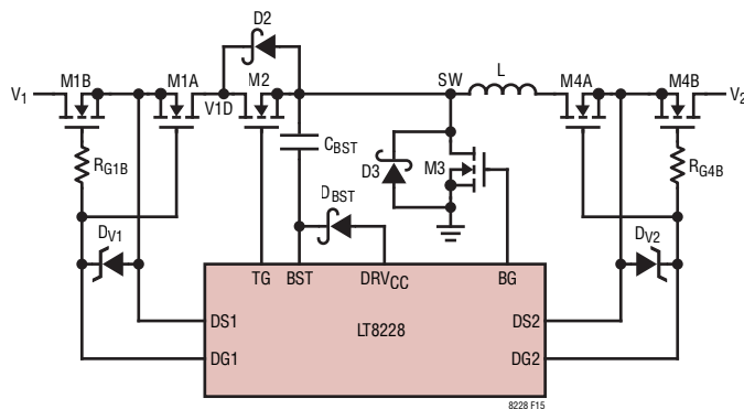
Figure 15. Power MOSFETs and Components Selection
