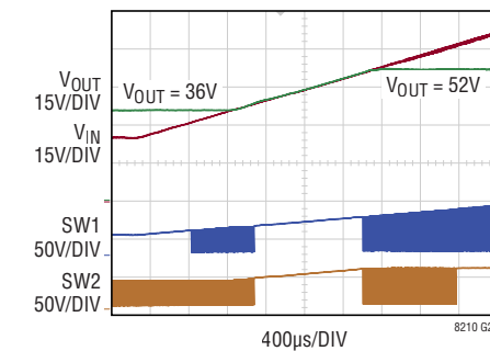
Input Voltage Sweep (Pass-Thru – Figure 37)
