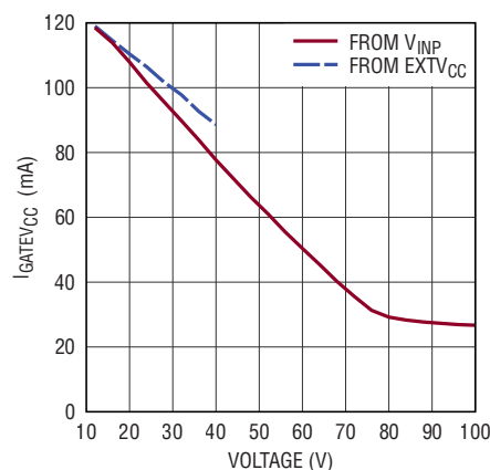
Figure 10. GATEV_{CC} Current Limit vs V_{INP} , EXTV_{CC}
