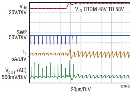
Line Step (Buck-Boost Region – Figure 37)
