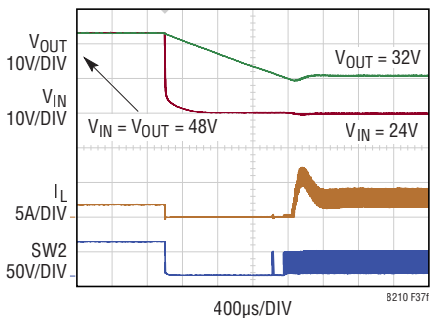
Pass-Thru Negative Surge (Falling Edge)
