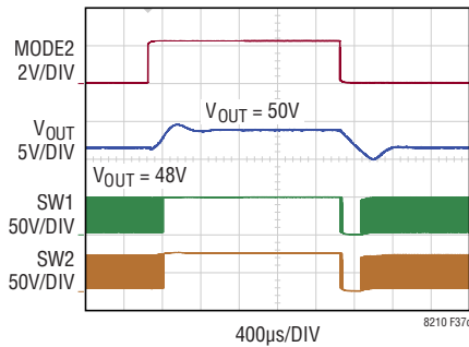
DCM to Pass-Thru Mode Transition ( V_{IN} = 50V )
