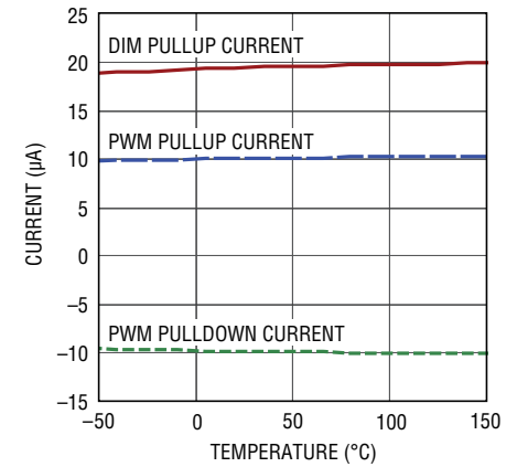
PWM Generator Currents vs Temperature
