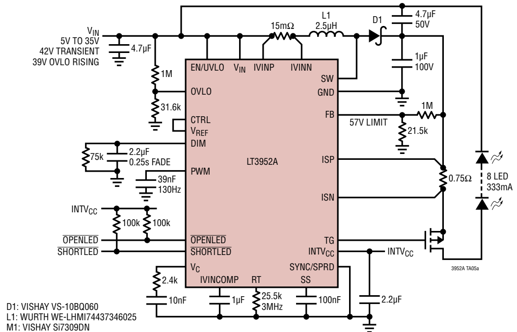
3MHz Buck-Boost LED Driver with Internal PWM Dimming and Fade Start
