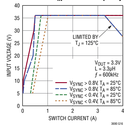
Maximum V_{IN} for Fixed Frequency
