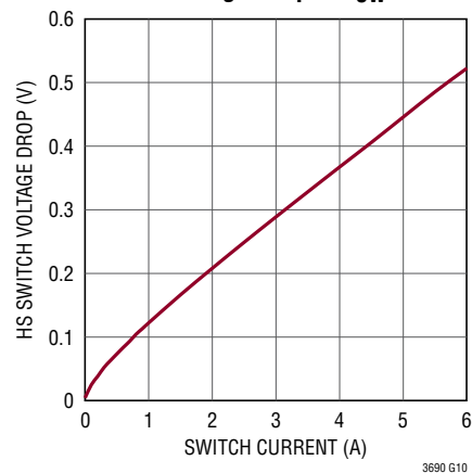
Switch Voltage Drop vs I_{SW}
