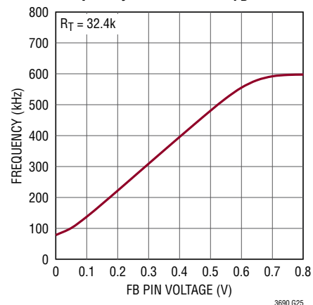
Frequency Foldback vs V_{FB}
