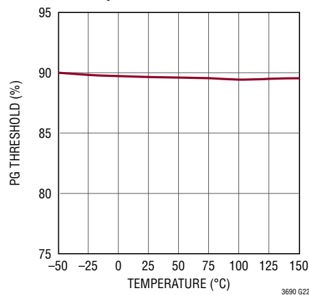
Power Good Threshold vs Temperature
