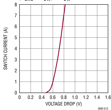
Catch Diode Voltage Drop ( V_{GND} - V_{SW} ) vs I_{SW}
