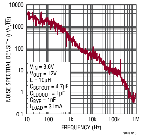
LT3048-12 LDOOUT Noise
