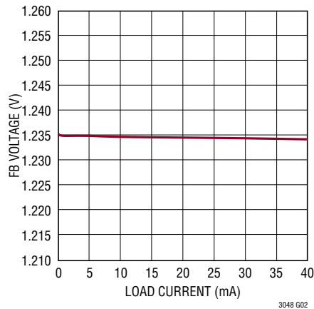
LT3048 FB Load Regulation
