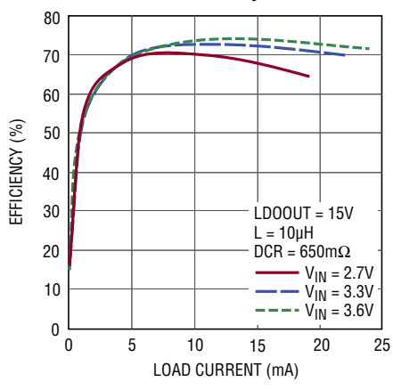
LT3048-15 Efficiency
