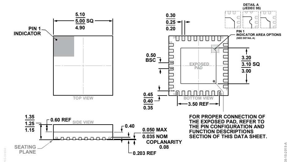
Figure 52. 32-Lead Lead Frame Chip Scale Package [LFCSP_CAV] 5 mm × 5 mm Body and 1.25 mm Package Height (CG-32-2)
