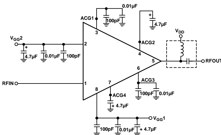
Figure 37. Application Circuit
