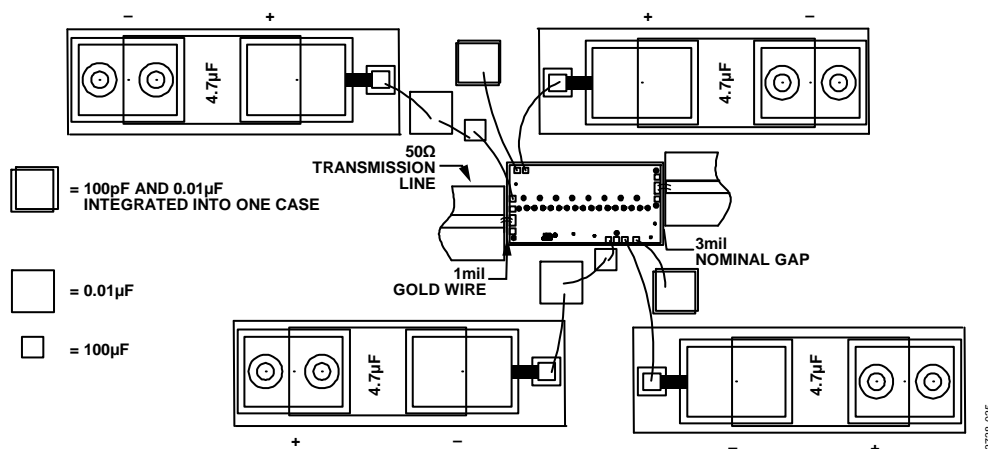
Figure 36. Assembly Diagram
