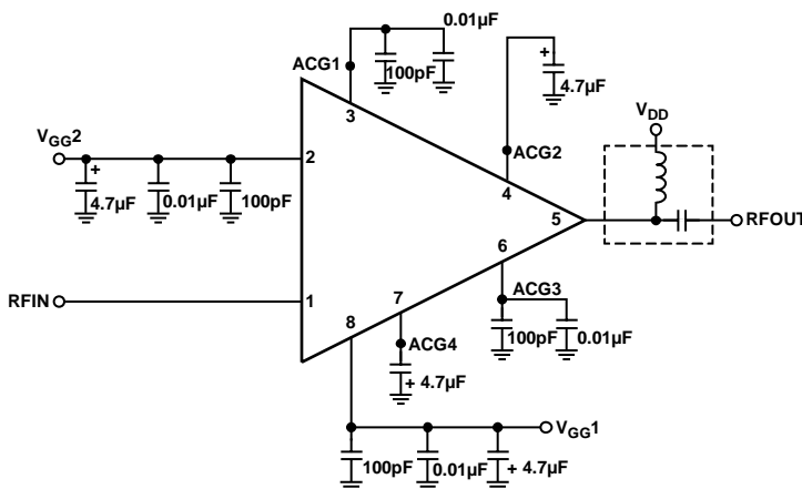
Figure 37. Application Circuit
