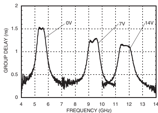
Group Delay, V_{ctl} = V_{bwctl}
