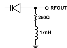
Figure 6. RFOUT Interface Schematic
