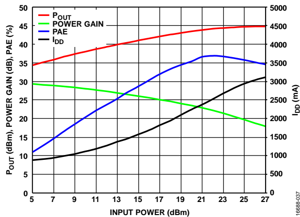
Figure 37. P_{OUT} , Power Gain, PAE, and I_{DD} vs. Input Power at 10.5 GHz
