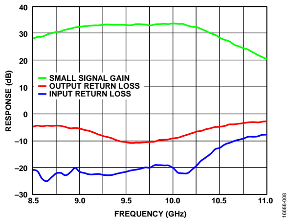
Figure 8. Small Signal Gain and Return Loss (Response) vs. Frequency
