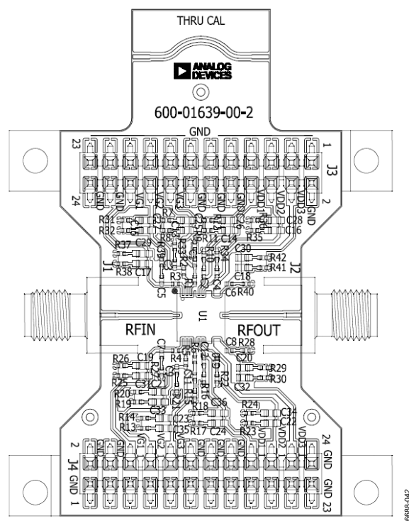
Figure 50. Evaluation PCB
