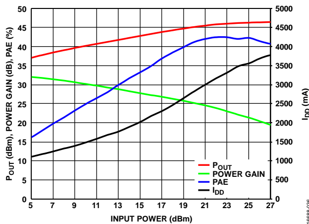
Figure 36. P_{OUT} , Power Gain, PAE, and I_{DD} vs. Input Power at 9.5 GHz
