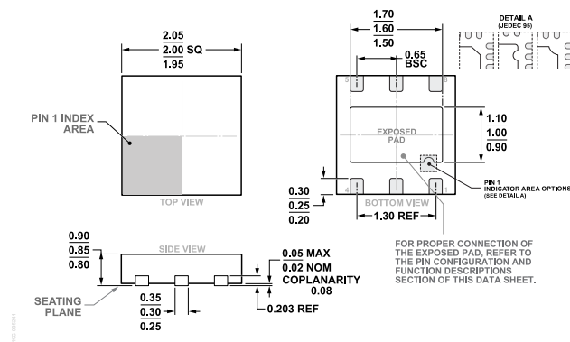
Figure 28. 6-Lead Lead Frame Chip Scale Package [LFCSP] 2 mm × 2 mm Body and 0.85 mm Package Height (CP-6-12) Dimensions shown in millimeters
