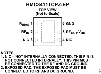
Figure 3. Pin Configuration
