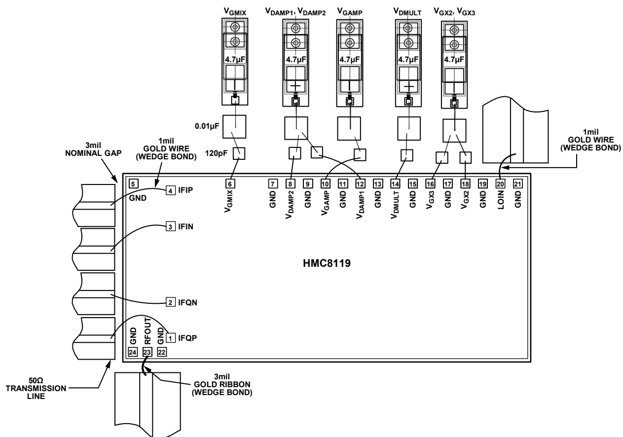
Figure 82. Assembly Diagram
