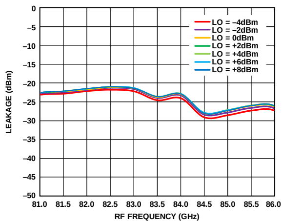
Figure 56. 6 \times LO Leakage at RFOUT vs. RF Frequency at Various LO Powers, I_{FIN} = 5 dBm, IF = 500 MHz, LSB
