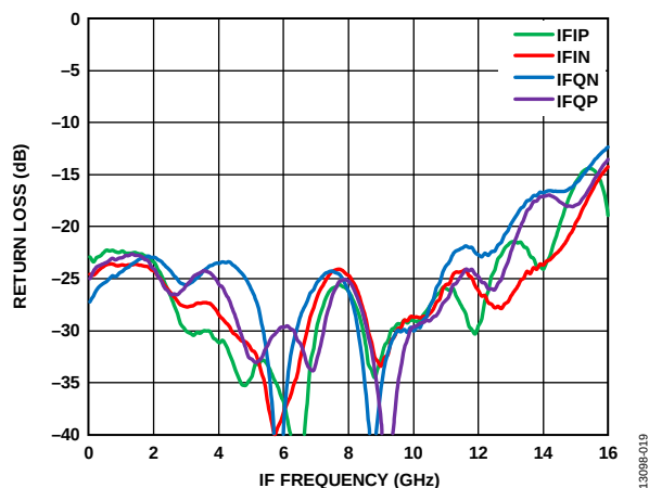
Figure 19. IF Return Loss vs. IF Frequency, LO = 2 dBm at 12 GHz
