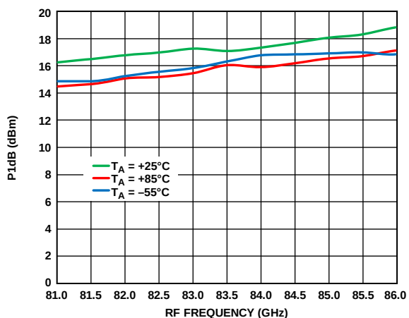
Figure 43. Input P1dB vs. RF Frequency at Various Temperatures, LO = 2 dBm, IF = 2000 MHz, USB
