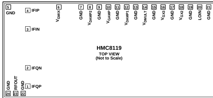
Figure 2. Pad Configuration
