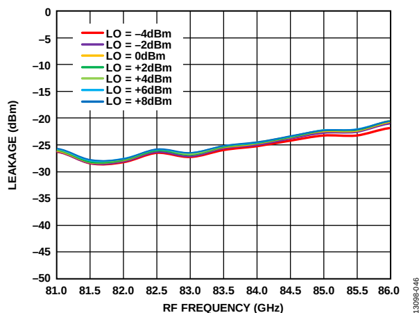
Figure 45. 6 \times LO Leakage at RFOUT vs. RF Frequency at Various LO Powers, I_{FIN} = 5 dBm, IF = 1000 MHz, USB
