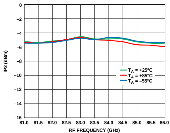
Figure 52. Input IP2 vs. RF Frequency at Various Temperatures, I_{FIN} = 5 dBm, LO = 2 dBm, IF = 500 MHz, LSB
