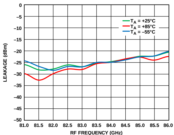
Figure 42. 6 \times LO Leakage at RFOUT vs. RF Frequency at Various Temperatures, I_{FIN} = 5 dBm, LO = 2 dBm, IF = 2000 MHz, USB
