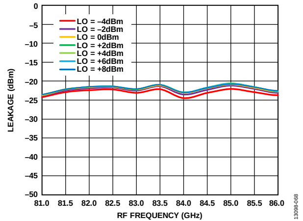
Figure 67. 6 \times LO Leakage at RFOUT vs. RF Frequency at Various LO Powers, I_{FIN} = 5 dBm, IF = 1000 MHz, LSB
