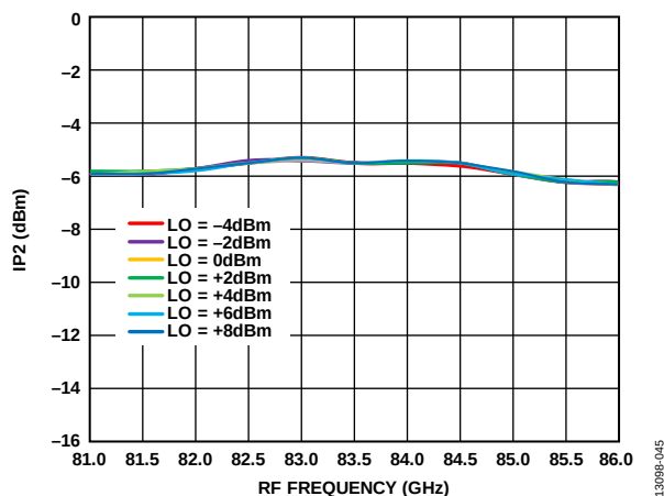
Figure 44. Input IP2 vs. RF Frequency at Various LO Powers, I_{FIN} = 5 dBm, IF = 2000 MHz, USB
