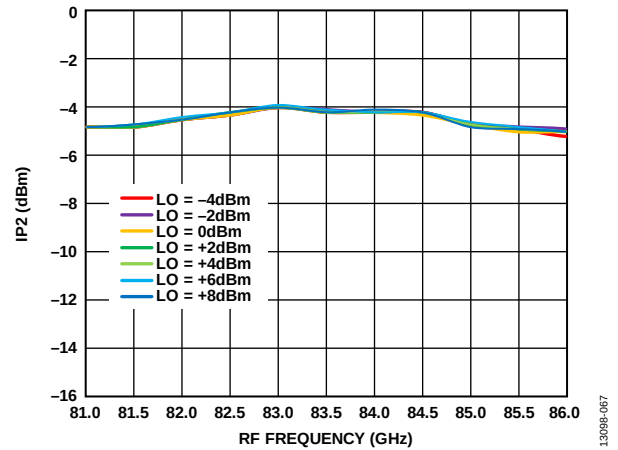
Figure 66. Input IP2 vs. RF Frequency at Various LO Powers, I_{FIN} = 5 dBm, IF = 1000 MHz, LSB
