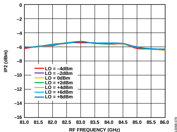
Figure 77. Input IP2 vs. RF Frequency at Various LO Powers, I_{FIN} = 5 dBm, IF = 2000 MHz, LSB
