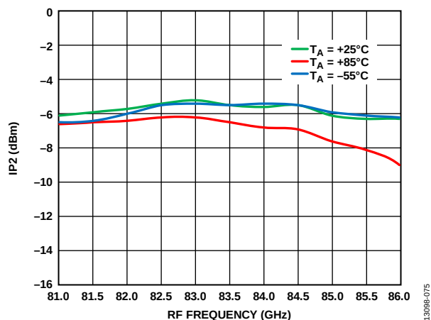
Figure 74. Input IP2 vs. RF Frequency at Various Temperatures, I_{FIN} = 5 dBm, LO = 2 dBm, IF = 2000 MHz, LSB
