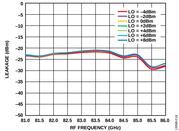
Figure 18. 6x LO Leakage at RFOUT vs. RF Frequency at Various LO Powers, IFIN = 5 dBm, IF = 500 MHz, USB
