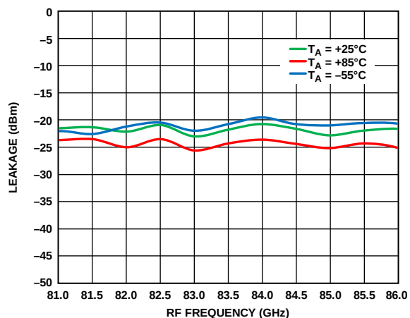
Figure 75. 6 \times LO Leakage at RFOUT vs. RF Frequency at Various Temperatures, I_{FIN} = 5 dBm, IF = 2000 MHz, LSB
