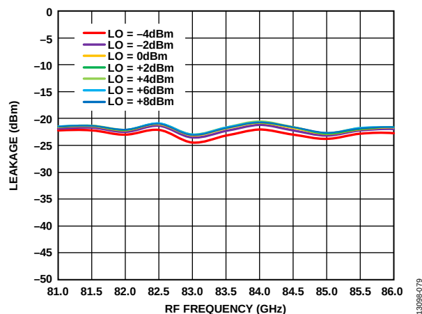
Figure 78. 6 \times LO Leakage at RFOUT vs. RF Frequency at Various LO Powers, I_{FIN} = 5 dBm, IF = 2000 MHz, LSB
