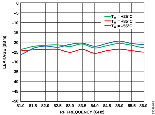
Figure 64. 6 \times LO Leakage at RFOUT vs. RF Frequency at Various Temperatures, I_{FIN} = 5 dBm, LO = 2 dBm, IF = 1000 MHz, LSB
