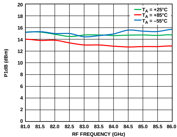
Figure 54. Input P1dB vs. RF Frequency at Various Temperatures, LO = 2 dBm, IF = 500 MHz, LSB
