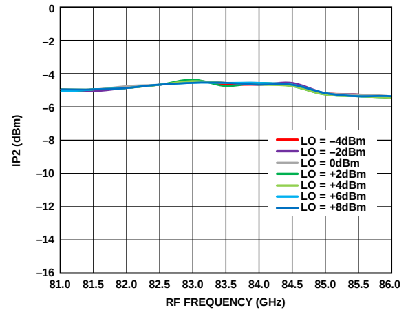
Figure 17. Input IP2 vs. RF Frequency at Various LO Powers, IFIN = 5 dBm, IF = 500 MHz, USB
