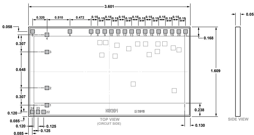
Figure 84. 24-Pad Bare Die [CHIP] (C-24-3)
