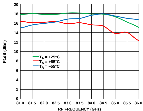
Figure 76. Input P1dB vs. RF Frequency at Various Temperatures, LO = 2 dBm, IF = 2000 MHz, LSB
