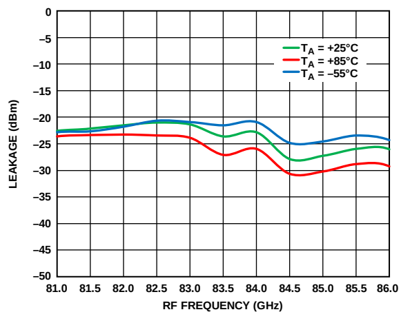
Figure 53. 6 \times LO Leakage at RFOUT vs. RF Frequency at Various Temperatures, I_{FIN} = 5 dBm, IF = 500 MHz, LSB
