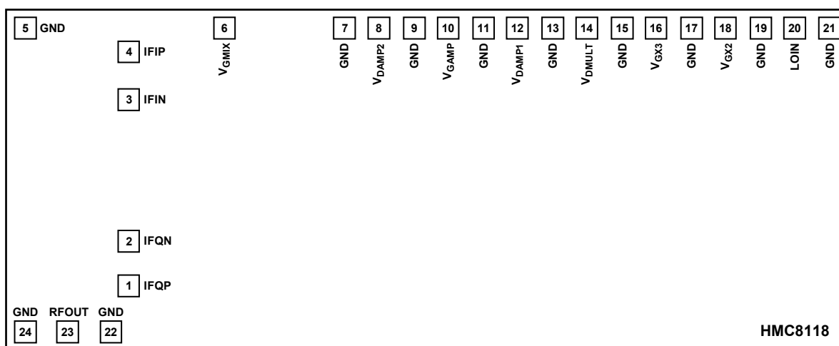
Figure 2. Pad Configuration
