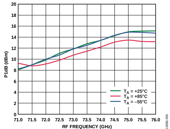
Figure 54. Input P1dB vs. RF Frequency at Various Temperatures, LO = 2 dBm, IF = 500 MHz, USB
