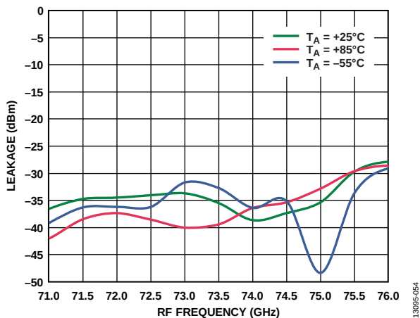
Figure 53. 6x LO Leakage at RFOUT vs. RF Frequency at Various Temperatures, I_{FIN} = 5 dBm, LO = 2 dBm, IF = 500 MHz, USB
