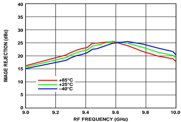
Figure 21. Image Rejection vs. RF Frequency over Temperature
