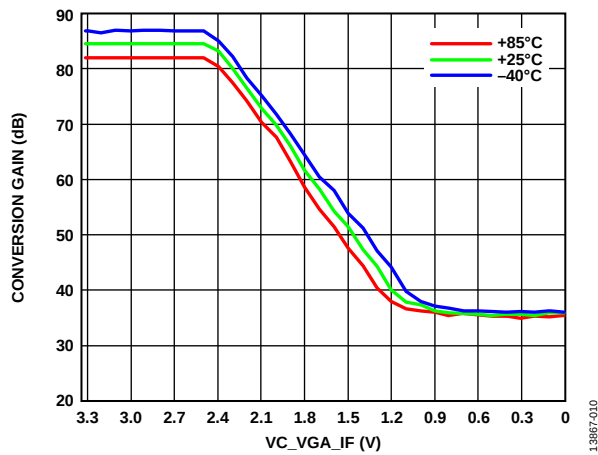
Figure 10. Conversion Gain vs. VC_VGA_IF at RF = 2 GHz, 56 MHz Filter (VC_VGA_RF = 3.3 V)
