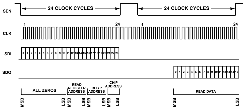
Figure 51. Timing Diagram, SPI Register Read
