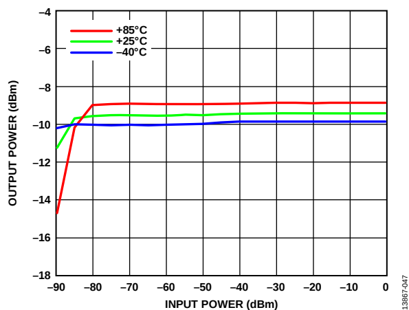
Figure 47. Output Power vs. Input Power over Temperature, RF = 4 GHz
