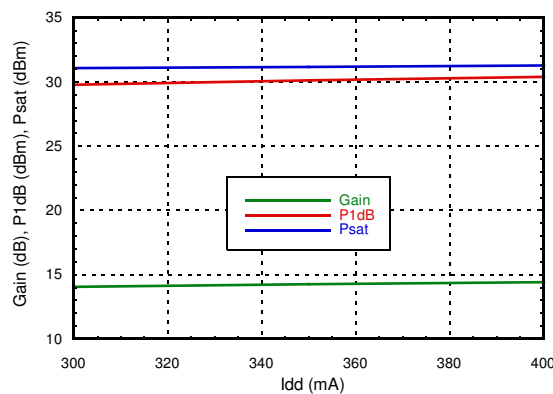
Gain & Power vs. Idd @ 10 GHz
