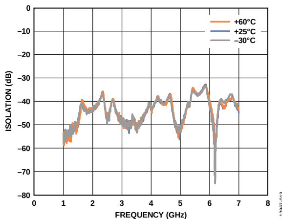
Figure 12. Reverse Isolation vs. Frequency at Various Temperatures
