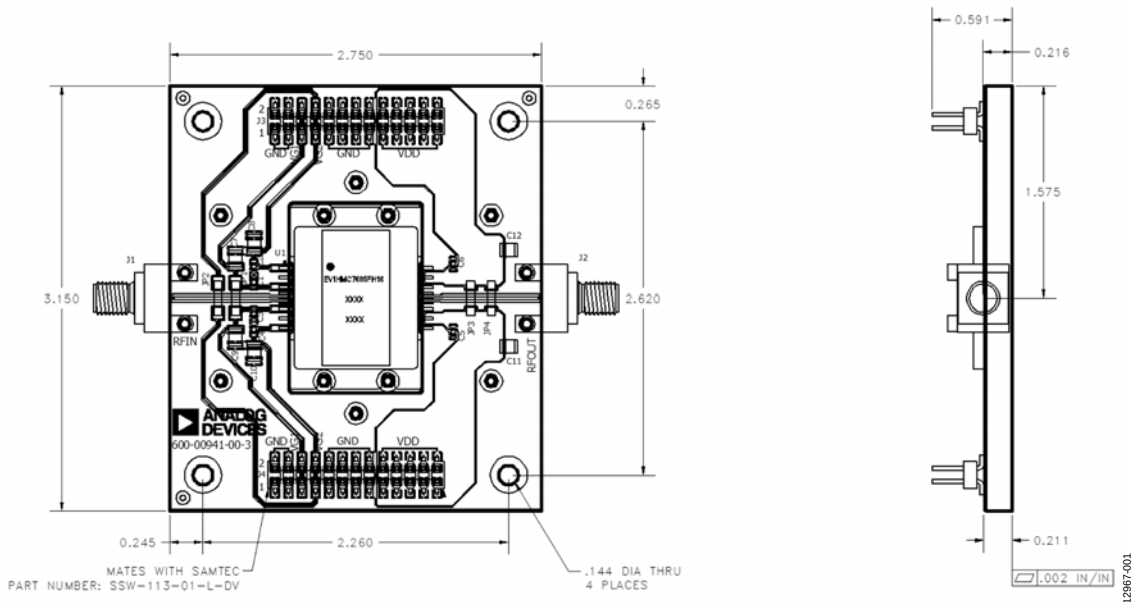
Figure 16. Evaluation Fixture
