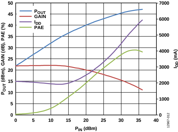
Figure 14. Power Compression at 4 GHz
