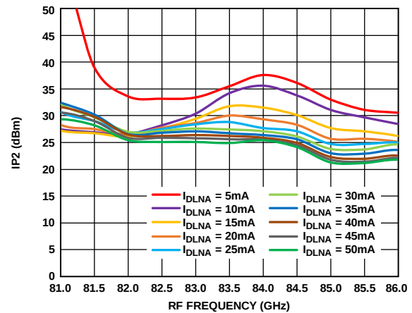
Figure 163. Input IP2 vs. RF Frequency at Various I_{DLNA} Values, R_{FIN} = -20 dBm, LO = 2 dBm, IF = 1000 MHz, V_{DLNA} = 3 V
