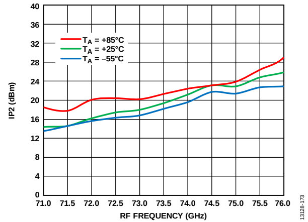
Figure 161. Input IP2 vs. RF Frequency at Various Temperatures, R_{FIN} = -20\text{ dBm} , LO = 2\text{ dBm} , IF = 1000\text{ MHz} , V_{DLNA} = 3\text{ V}
