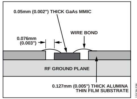
Figure 214. Routing RF Signals
