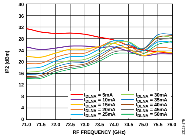
Figure 163. Input IP2 vs. RF Frequency at Various I_{DLNA} Values, R_{FIN} = -20\text{ dBm} , LO = 2\text{ dBm} , IF = 1000\text{ MHz} , V_{DLNA} = 3\text{ V}
