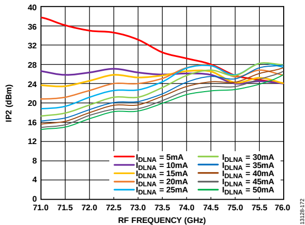
Figure 160. Input IP2 vs. RF Frequency at Various I_{DLNA} Values, R_{FIN} = -20\text{ dBm} , LO = 2\text{ dBm} , IF = 1000\text{ MHz} , V_{DLNA} = 4\text{ V}
