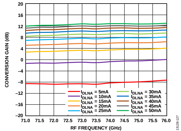
Figure 119. Conversion Gain vs. RF Frequency at Various I_{DLNA} Values, R_{FIN} = -20 dBm, IF = 500 MHz, V_{DLNA} = 3 V
