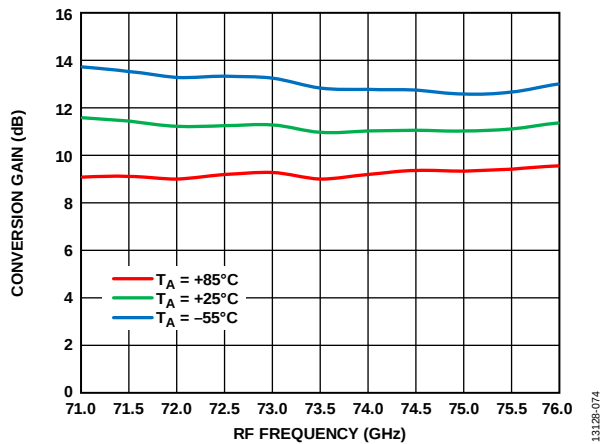
Figure 70. Conversion Gain vs. RF Frequency at Various Temperatures, R_{FIN} = -20\text{ dBm} , LO = 2\text{ dBm} , IF = 2000\text{ MHz} , V_{DLNA} = 4\text{ V}
