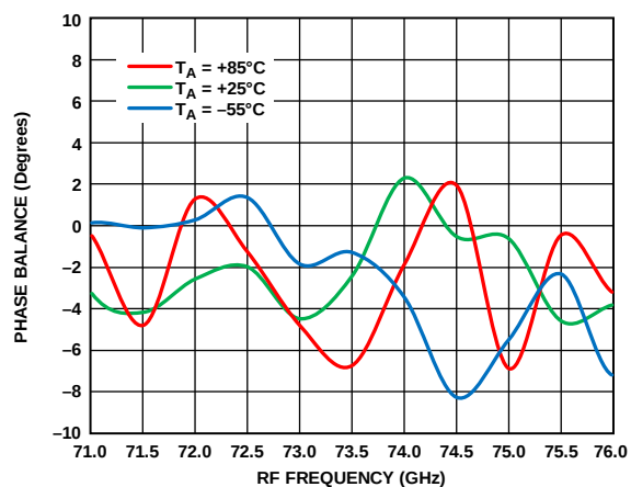
Figure 208. Phase Balance vs. RF Frequency at Various Temperatures, RFIN = -20 dBm, LO = 2 dBm, IF = 1000 MHz, V_{DLN} = 3 V
