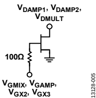
Figure 5. V_{DAMP1} , V_{DAMP2} , V_{DMULT} , V_{GAMP} , V_{GMIX} , V_{GX2} , and V_{GX3} Interface
