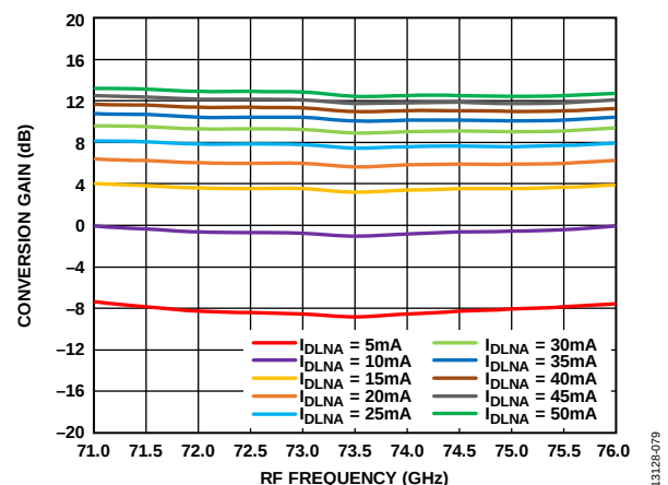
Figure 75. Conversion Gain vs. RF Frequency at Various I_{DLNA} Values, R_{FIN} = -20\text{ dBm} , IF = 2000\text{ MHz} , V_{DLNA} = 3\text{ V}
