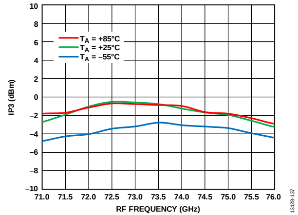
Figure 129. Input IP3 vs. RF Frequency at Various Temperatures, RFIN = -20 dBm, LO = 2 dBm, IF = 500 MHz, V_{DLNA} = 3 V
