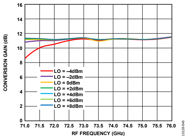
Figure 45. Conversion Gain vs. RF Frequency at Various LO Powers, R_{FIN} = -20\text{ dBm} , IF = 500\text{ MHz} , V_{DLNA} = 4\text{ V}
