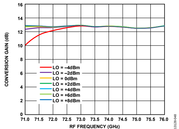
Figure 48. Conversion Gain vs. RF Frequency at Various LO Powers, R_{FIN} = -20\text{ dBm} , IF = 500\text{ MHz} , V_{DLNA} = 3\text{ V}
