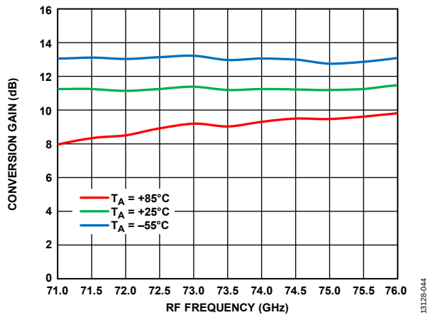
Figure 44. Conversion Gain vs. RF Frequency at Various Temperatures, R_{FIN} = -20\text{ dBm} , LO = 2\text{ dBm} , IF = 500\text{ MHz} , V_{DLNA} = 4\text{ V}
