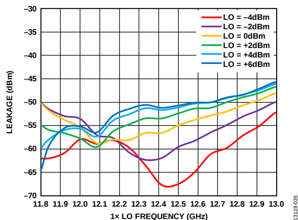
Figure 35. LO Leakage at IFOUT vs. 1x LO Frequency at Various LO Powers, V_{DLNA} = 3 V
