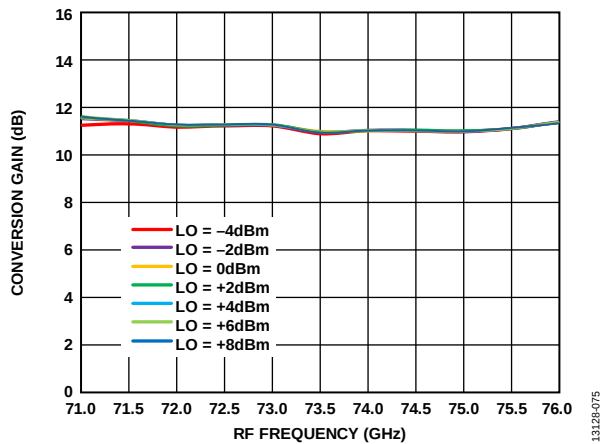
Figure 71. Conversion Gain vs. RF Frequency at Various LO Powers, R_{FIN} = -20\text{ dBm} , IF = 2000\text{ MHz} , V_{DLNA} = 4\text{ V}
