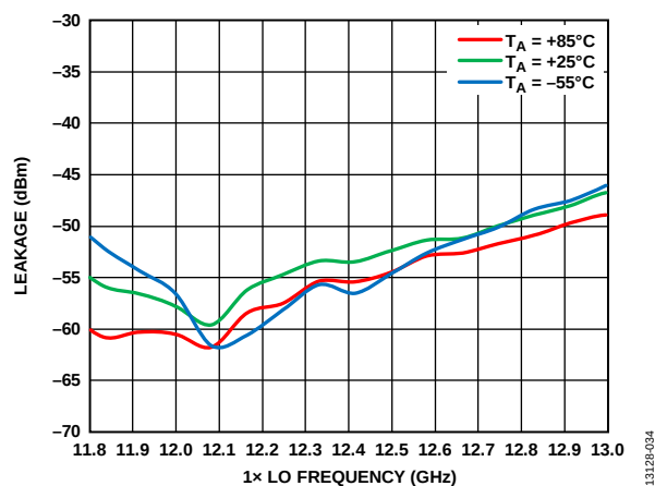
Figure 34. LO Leakage at IFOUT vs. 1x LO Frequency at Various Temperatures, LO = 2 dBm, V_{DLNA} = 3 V
