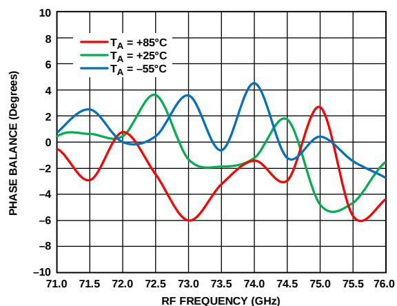
Figure 207. Phase Balance vs. RF Frequency at Various Temperatures, RFIN = -20 dBm, LO = 2 dBm, F = 500 MHz, V_{DLN} = 3 V
