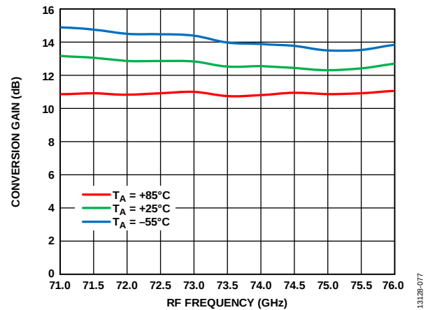
Figure 73. Conversion Gain vs. RF Frequency at Various Temperatures, R_{FIN} = -20\text{ dBm} , LO = 2\text{ dBm} , IF = 2000\text{ MHz} , V_{DLNA} = 3\text{ V}
