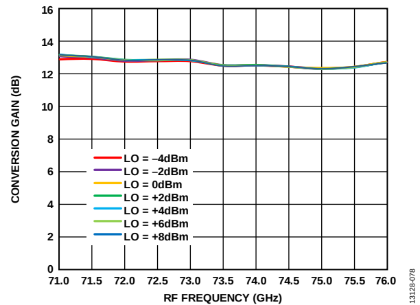
Figure 74. Conversion Gain vs. RF Frequency at Various LO Powers, R_{FIN} = -20\text{ dBm} , IF = 2000\text{ MHz} , V_{DLNA} = 3\text{ V}
