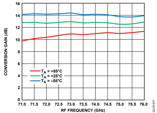
Figure 47. Conversion Gain vs. RF Frequency at Various Temperatures, R_{FIN} = -20\text{ dBm} , LO = 2\text{ dBm} , IF = 500\text{ MHz} , V_{DLNA} = 3\text{ V}
