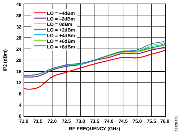
Figure 159. Input IP2 vs. RF Frequency at Various LO Powers, R_{FIN} = -20\text{ dBm} , IF = 1000\text{ MHz} , V_{DLNA} = 4\text{ V}
