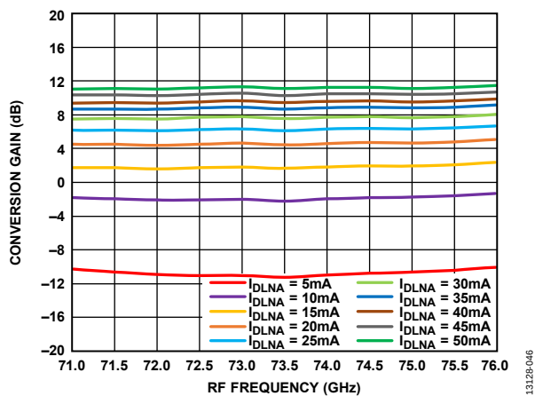
Figure 46. Conversion Gain vs. RF Frequency at Various I_{DLNA} Values, R_{FIN} = -20\text{ dBm} , IF = 500\text{ MHz} , V_{DLNA} = 4\text{ V}
