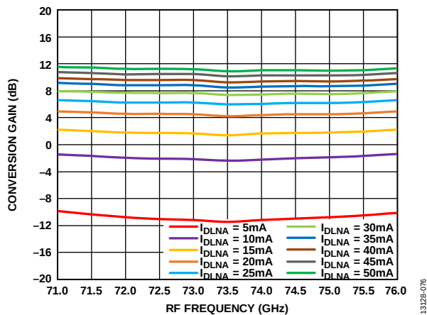
Figure 72. Conversion Gain vs. RF Frequency at Various I_{DLNA} Values, R_{FIN} = -20\text{ dBm} , IF = 2000\text{ MHz} , V_{DLNA} = 4\text{ V}
