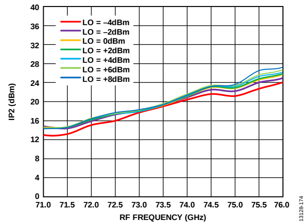
Figure 162. Input IP2 vs. RF Frequency at Various LO Powers, R_{FIN} = -20\text{ dBm} , IF = 1000\text{ MHz} , V_{DLNA} = 3\text{ V}
