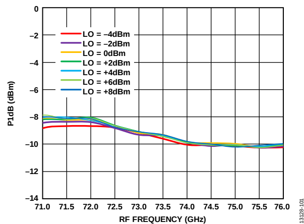
Figure 95. Input P1dB vs. RF Frequency at Various LO Powers, IF = 2000 MHz, V_{DLNA} = 4\text{ V}
