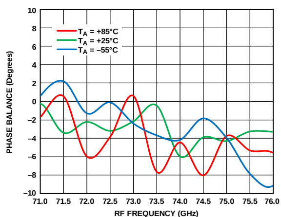
Figure 209. Phase Balance vs. RF Frequency at Various Temperatures, RFIN = -20 dBm, LO = 2 dBm, IF = 2000 MHz, V_{DLN} = 3 V
