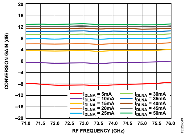
Figure 49. Conversion Gain vs. RF Frequency at Various I_{DLNA} Values, R_{FIN} = -20\text{ dBm} , IF = 500\text{ MHz} , V_{DLNA} = 3\text{ V}
