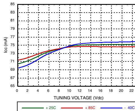
Supply Current
