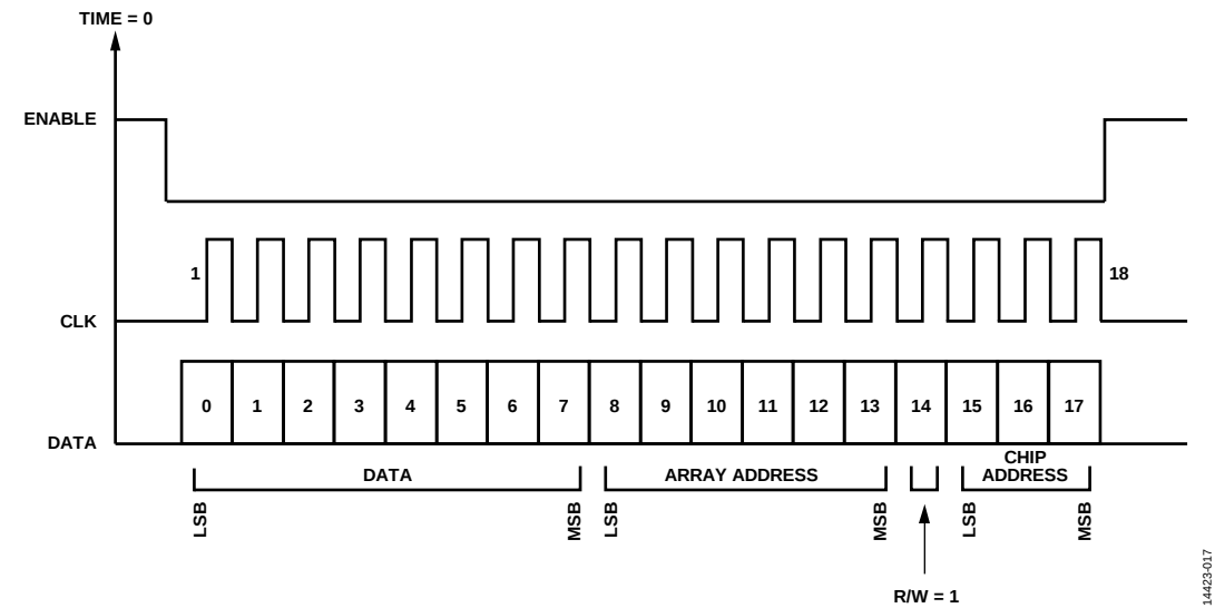
Figure 17. Timing Diagram for Writing a Row of the Transmitter Serial Interface
