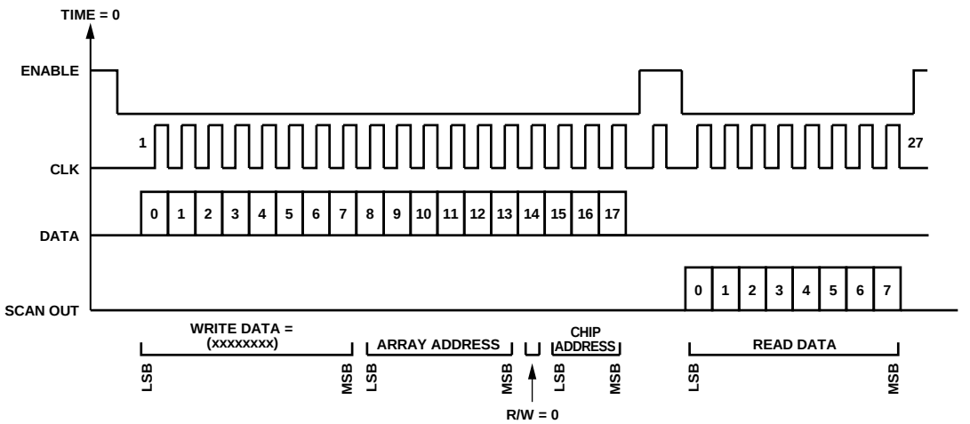
Figure 18. Timing Diagram for Reading a Row of the Transmitter Serial Interface
